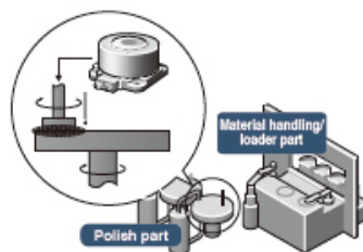
[Rotary axis for polishing systems]
